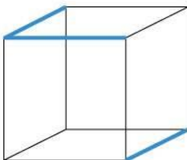
ARESTA
